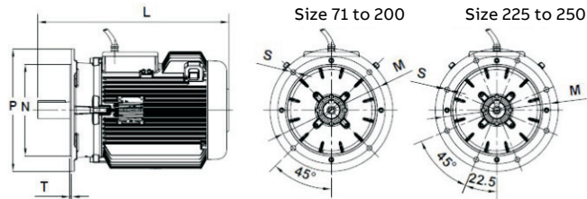
Flange mounted motor IM3001, B5 (TEAO)
