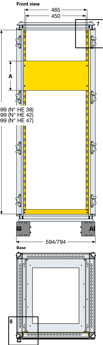
Fixed rack frame
