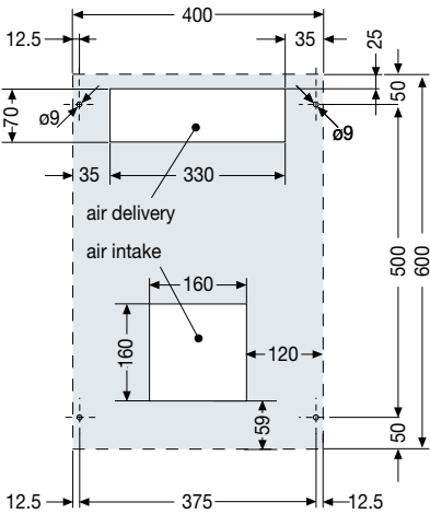
Drilling template
