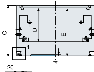
Modular panels and internal counterdoor
