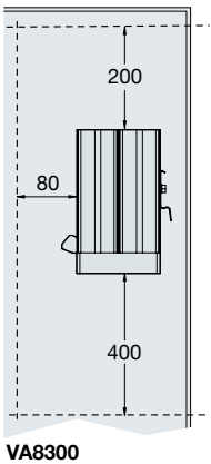
Minimum mounting distances
