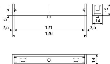
Clip for wiring ducts base 120
