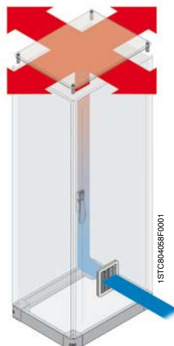
Natural aeration with roof lifting kit (IP20) and grating.
