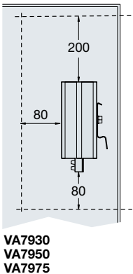
Minimum mounting distances
