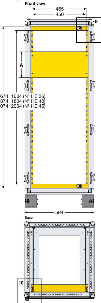
Swing rack frame W=600mm
